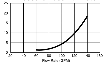
Pressure Loss Ft. Water
